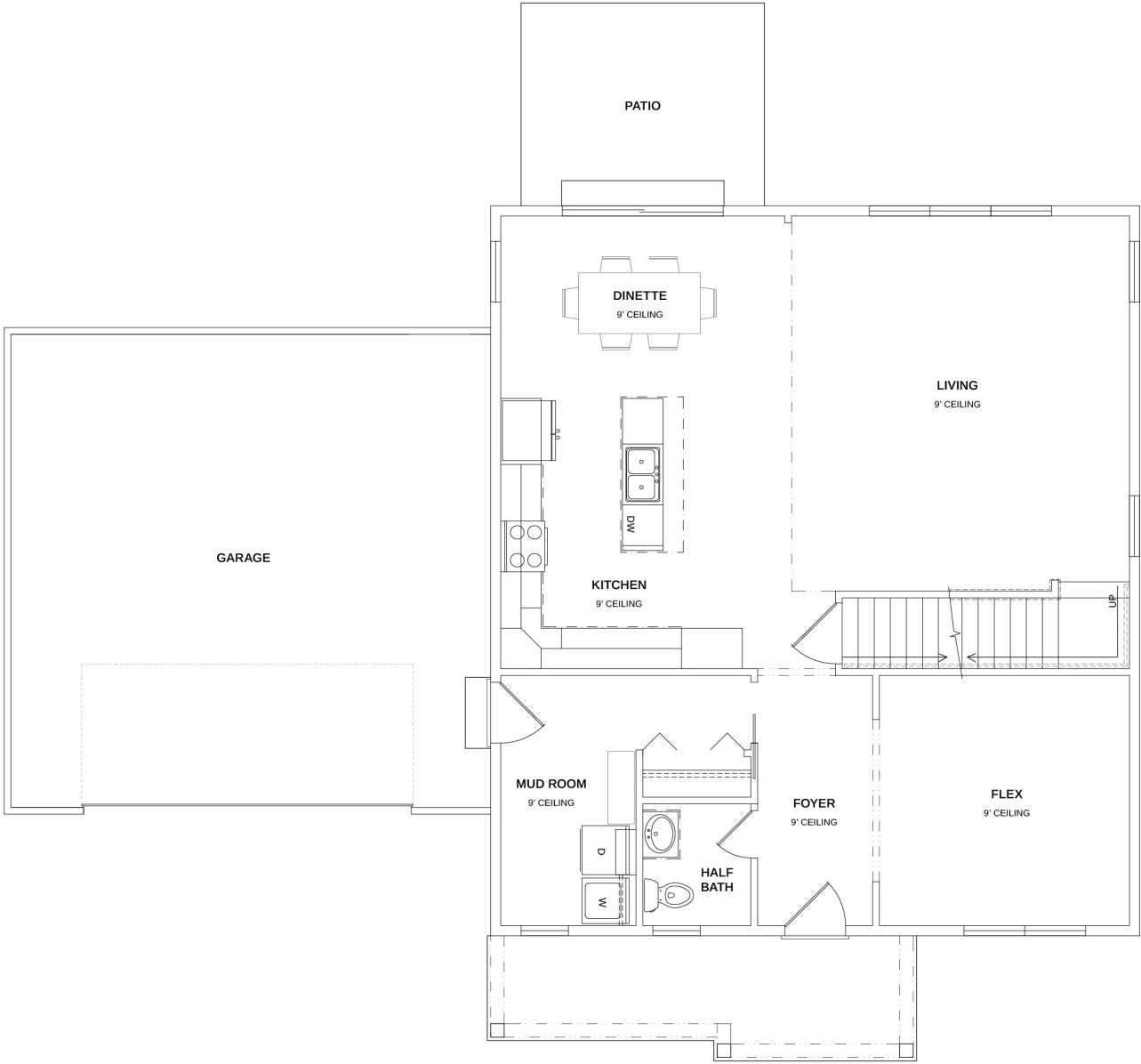
CHARLESTON MAIN FLOOR PLAN
