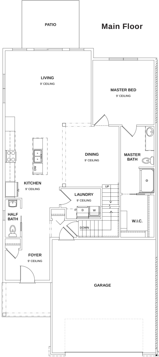
HAMPTON FLOOR PLANS
