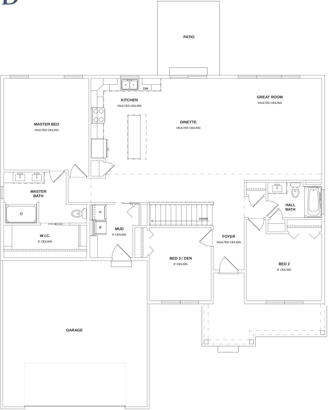
KOHEN FLOOR PLAN
