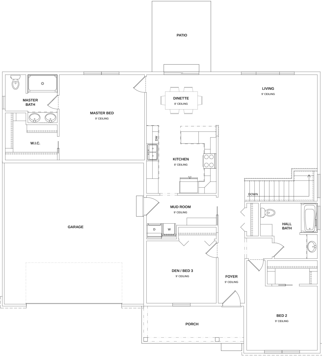
STRATFORD FLOOR PLAN
